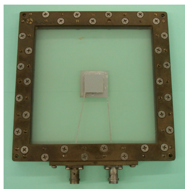
Fig.2 Appearance of an ionization chamber
