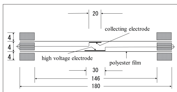
Fig.1 Cross section of an ionization chamber
