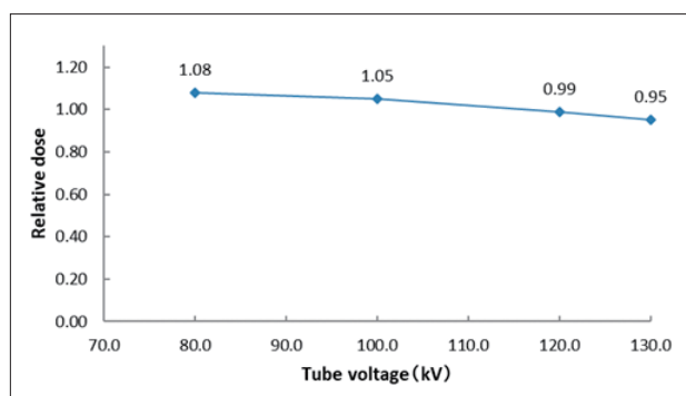
Fig.10 Beam quality dependence of an ionization chamber
