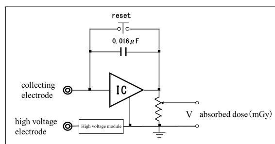
Fig.3 Principle of measuring circuit of an amplifier
